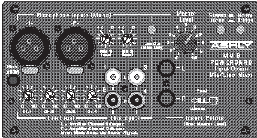
Figure 8.4: MM-6 Mic - Line Mixer
