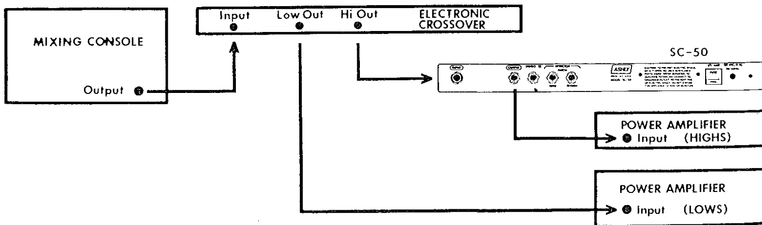
Figure 24 Alternate biamplification approach.
