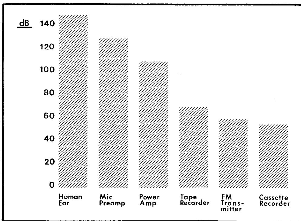
Figure 7 Comparison of the dynamic range of several common audio systems.
