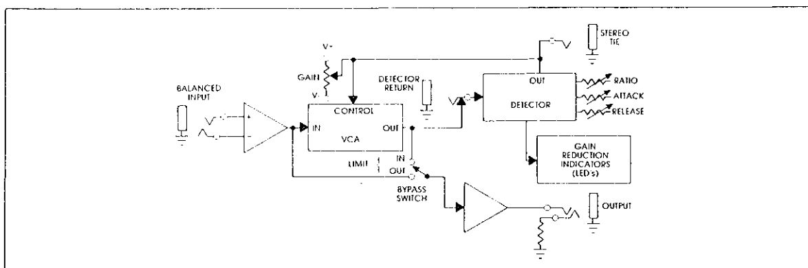
SC-50 BLOCK DIAGRAM
