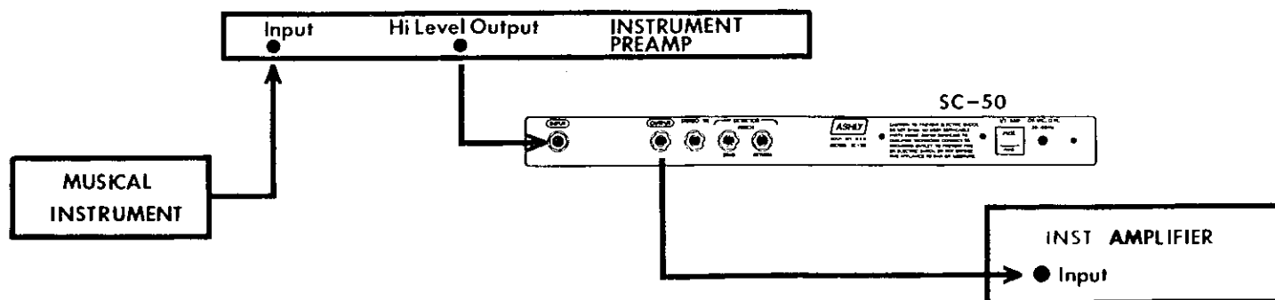
Figure 30 The SC-50 used with a musical instrument preamplifier.
