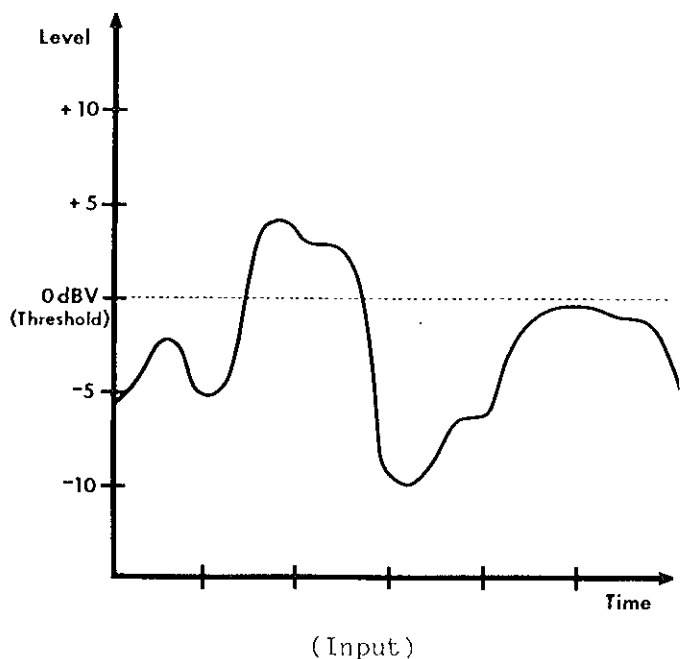
Figure 20 LIMITING. Once the Input level begins to exceed threshold, limiting will begin to occur. Notice that the Output is an exact copy of the Input for all signals which are below threshold. Only the signal peak which exceeded threshold has been gain reduced, in this case by a 4:1 ratio.
