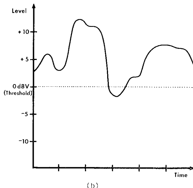
Figure 19 The constantly changing loudness levels of a typical musical program. The over-all volume level of the signal on the right is greater; it is above threshold most of the time. This is in contrast to the graph on the left (a), where the loudest volume peak just barely reaches threshold.
