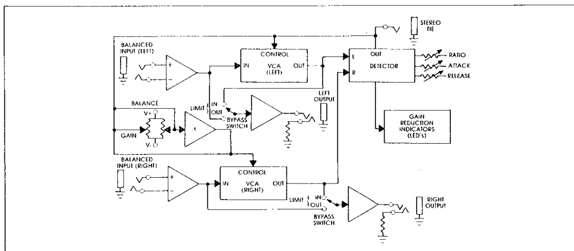
SC-55 BLOCK DIAGRAM
