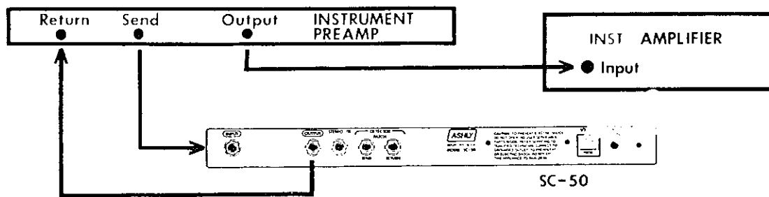
Figure 31 The SC-50 inserted into the effects loop of a musical instrument preamplifier.
