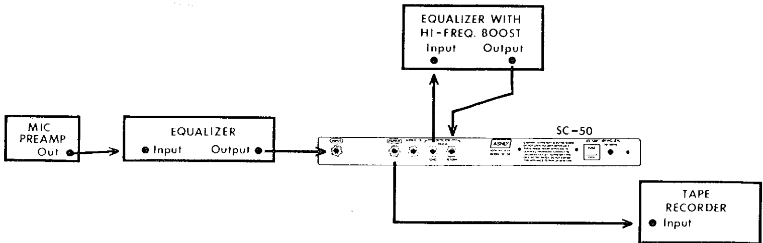
Figure 27 "De-Essing" with the SC-50.
