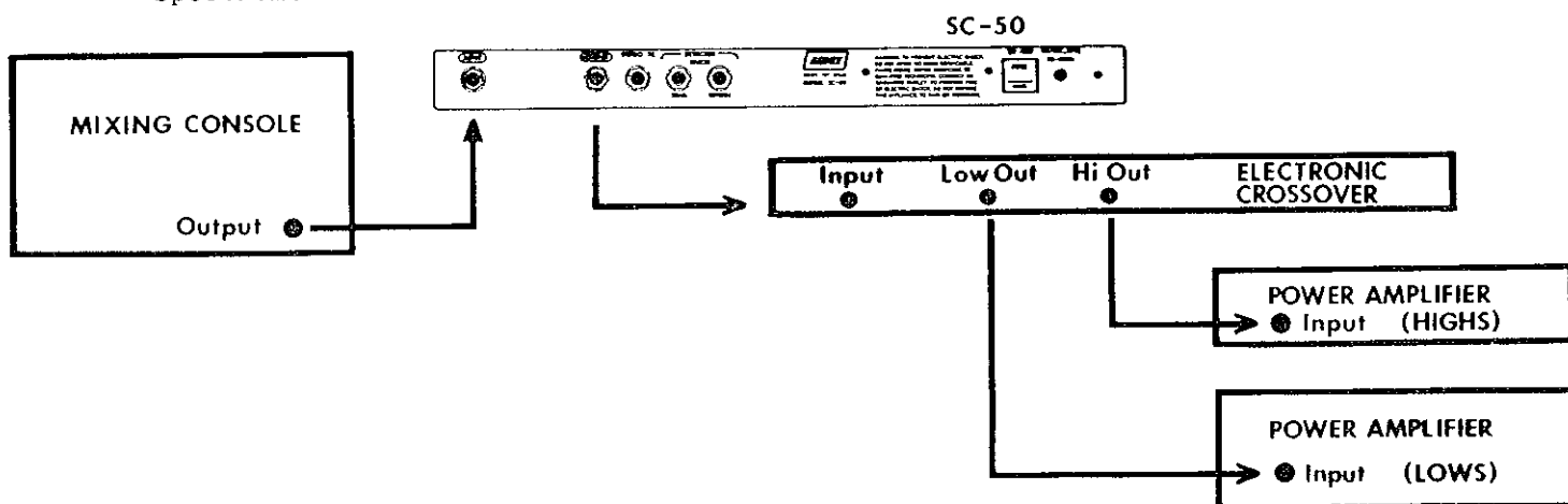
Figure 23 The SC-50 in a biamplified system.
