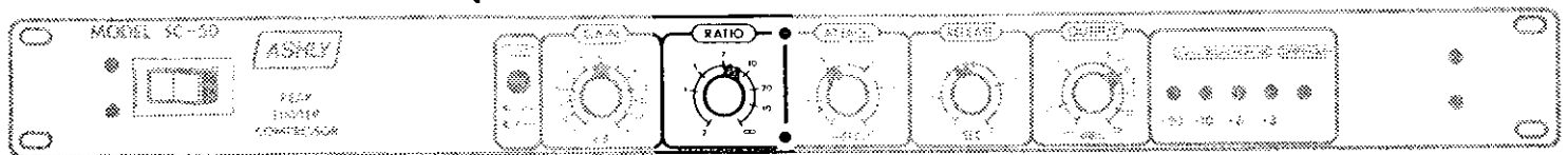
Figure 11 The Ashly SC-50 and SC-55 provide continuously variable RATIO control from 2:1 to infinity.
