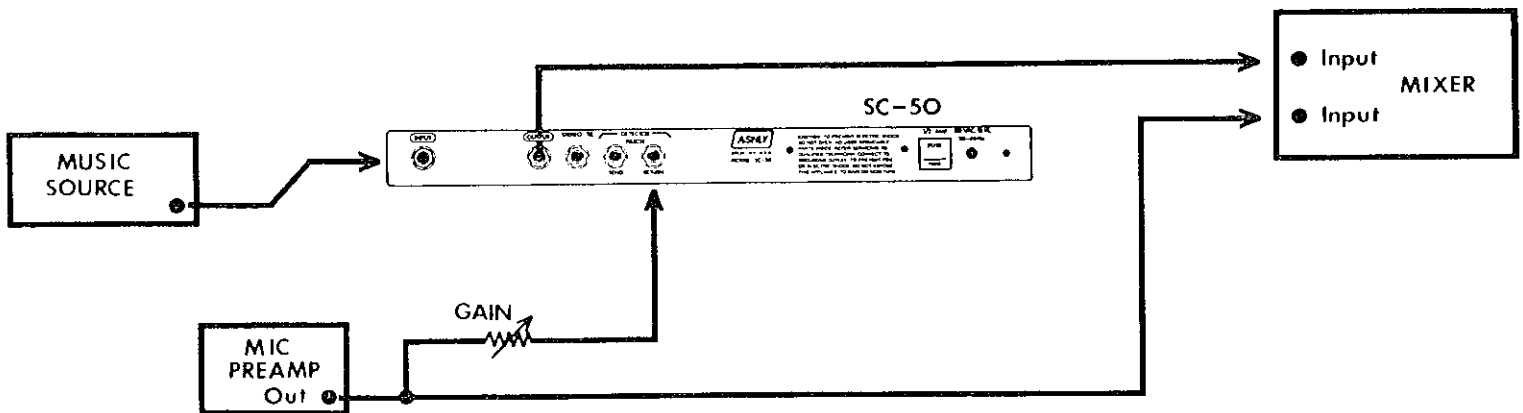
Figure 32 The SC-50 as a "Voice-Over" Compressor.
