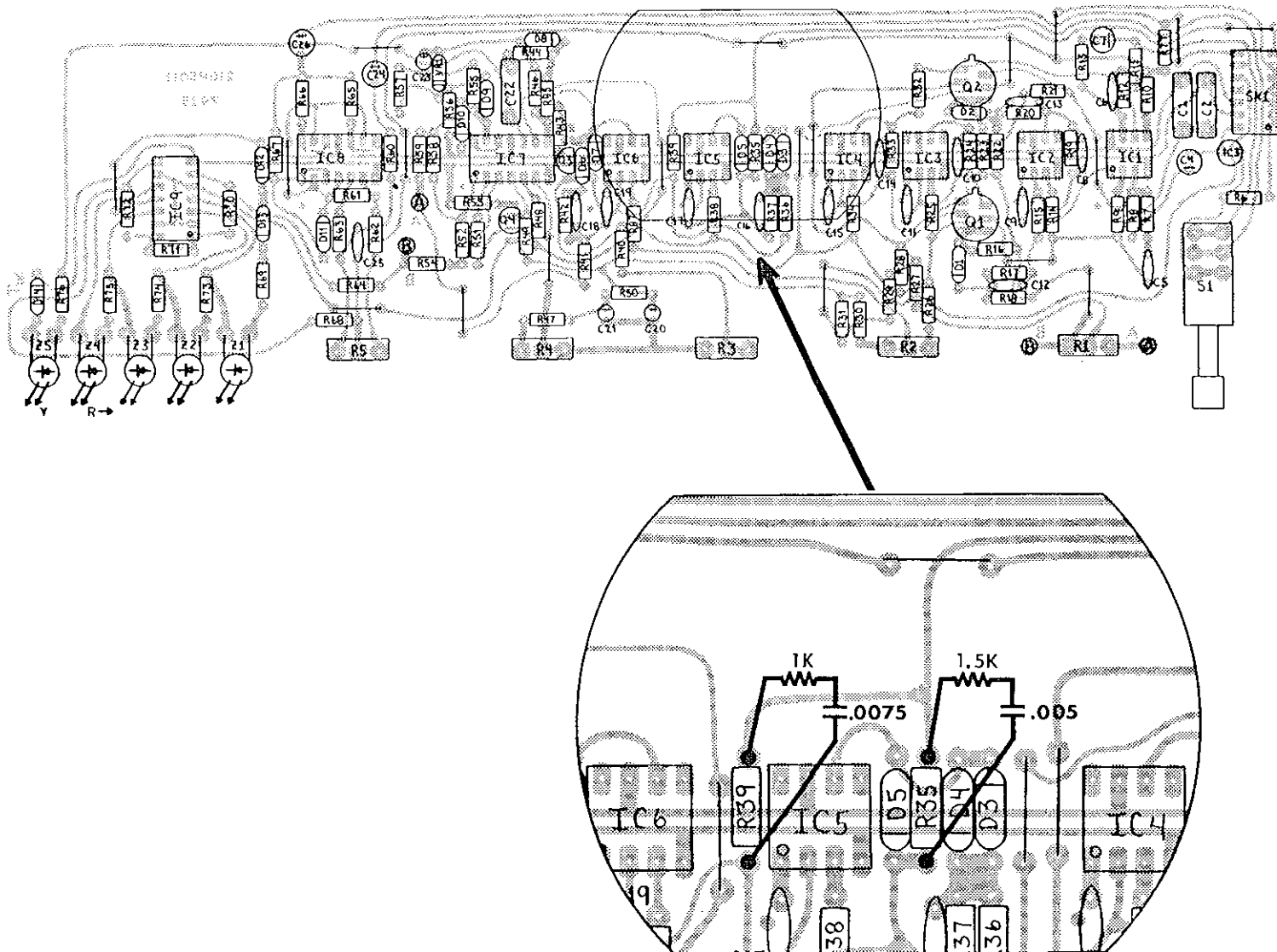
Figure 28 FM Pre-emphasis modification, SC-50. Capacitor values shown are for 75 microsecond pre-emphasis. For 25 microsecond values (Dolby), see the table below.
