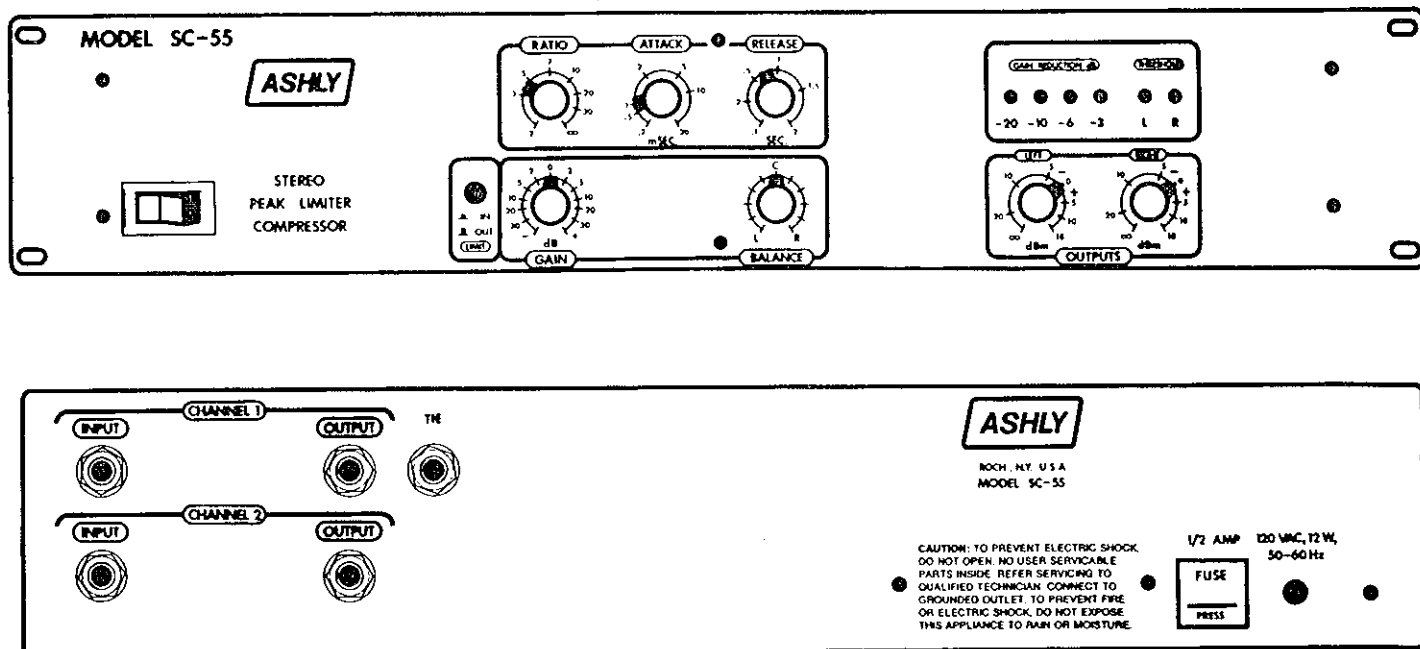
Figure 2 SC-55 front and back panels.
