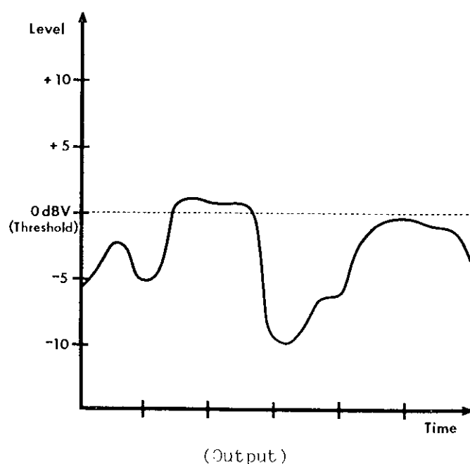
Figure 20 LIMITING. Once the Input level begins to exceed threshold, limiting will begin to occur. Notice that the Output is an exact copy of the Input for all signals which are below threshold. Only the signal peak which exceeded threshold has been gain reduced, in this case by a 4:1 ratio.
