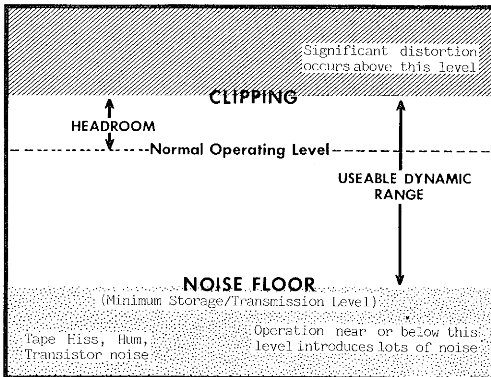
Figure 8 The useful dynamic range of any piece of audio equipment is limited by noise and distortion.
