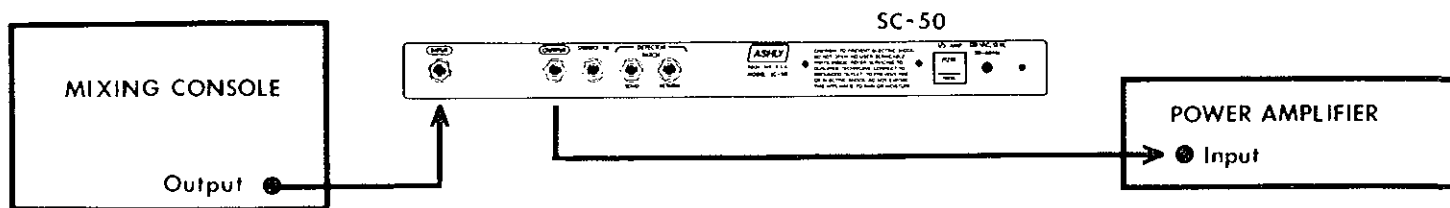
Figure 22 Installing the SC-50 for use in a sound system with a passive crossover.
