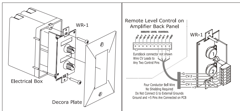
4.1 - WR-1 Assembly and Wiring
