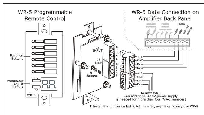
4.4 - WR-5 Wiring
