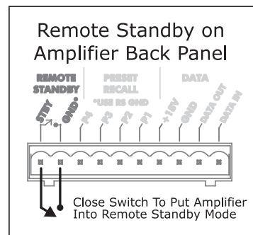
Remote Standby Contact Closure Wiring
