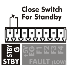
6.3 Standby Circuit
