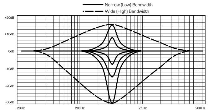
ne24.24M Parametric Filters
