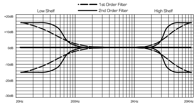
ne24.24M Shelving Filters
