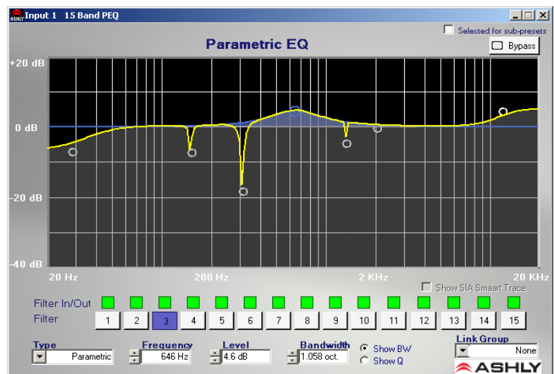
ne24.24M Parametric Filters
